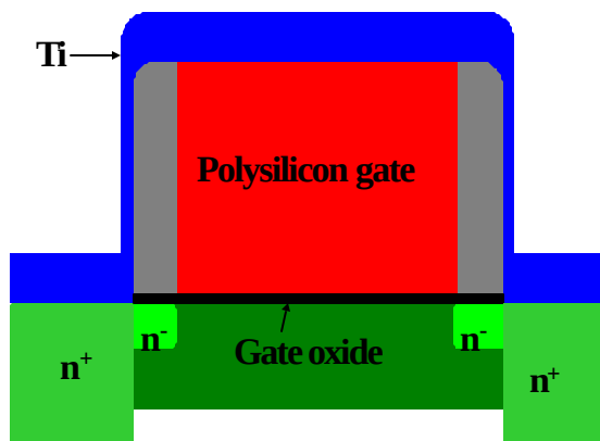
Titanium deposition
